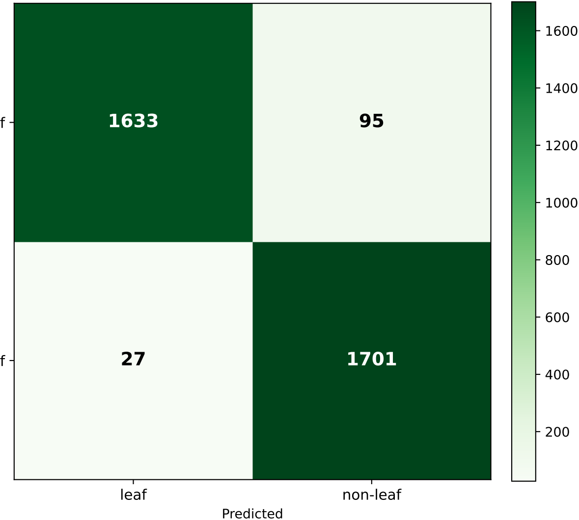
Confusion matrix — clean PyTorch FP32 test
